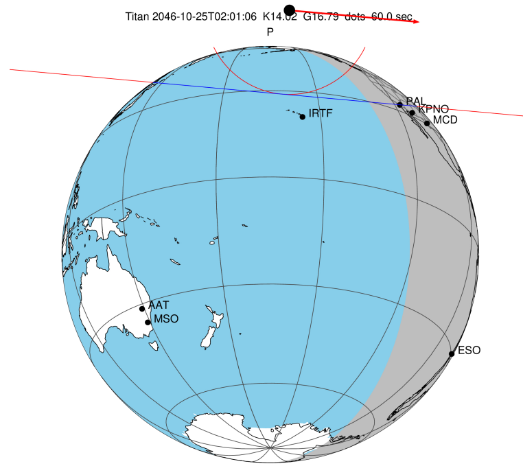
2046-10-25T02:01:06.7200 α: 17 13 16.8908 δ: -21 48 27.047 C/A 0.967" PA 5.18 deg v_sky +34.93 km/s D 10.69 AU Credit: Styled after SORA/Lucky Star
