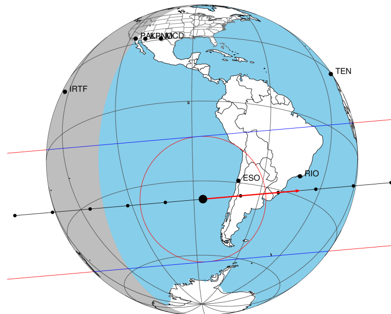
2047-02-08T14:36:23.3800 α: 18 03 21.4174 δ: -22 23 13.422 C/A 0.206" PA 174.96 deg v_sky +25.75 km/s D 10.67 AU Credit: Styled after SORA/Lucky Star
