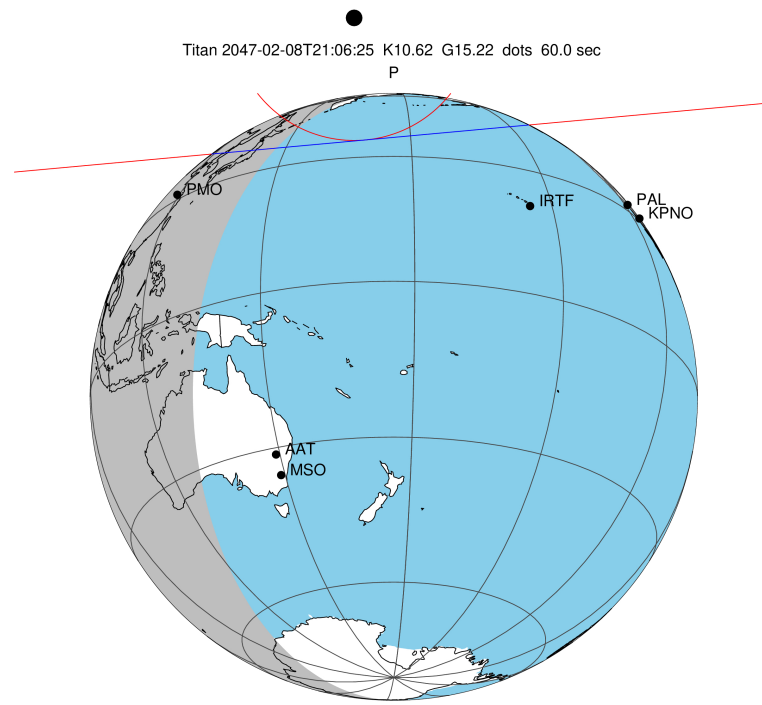
2047-02-08T21:06:25.4200 α: 18 03 27.0571 δ: -22 23 07.640 C/A 1.035" PA 354.77 deg v_sky +26.10 km/s D 10.67 AU Credit: Styled after SORA/Lucky Star
