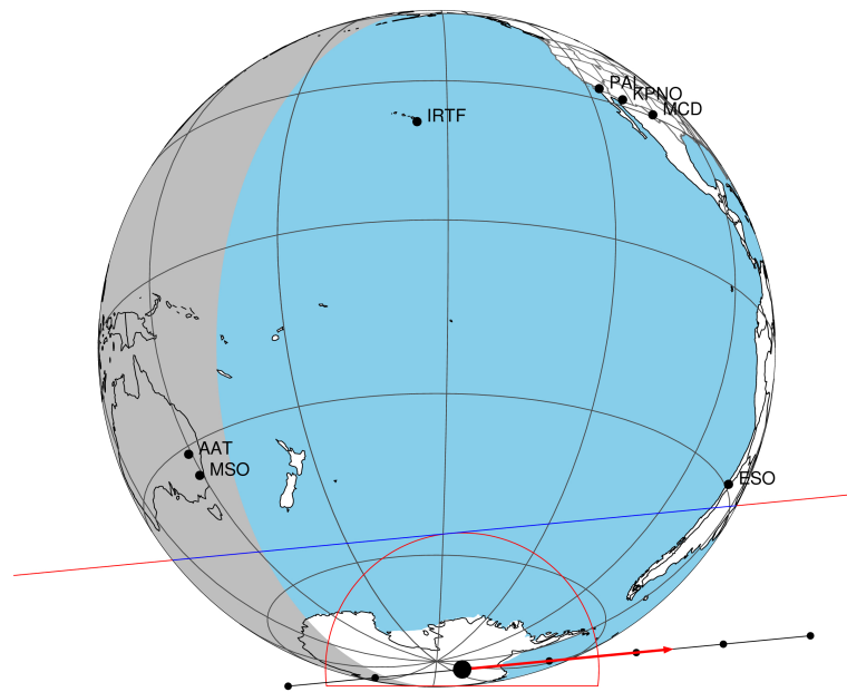
2047-02-09T18:55:07.1300 α: 18 03 46.5506 δ: -22 22 40.079 C/A 0.785" PA 174.49 deg v_sky +27.46 km/s D 10.66 AU Credit: Styled after SORA/Lucky Star
