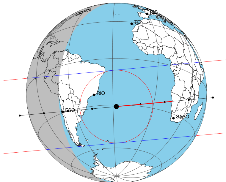
2047-02-10T10:34:53.2400 α: 18 04 01.2181 δ: -22 22 21.319 C/A 0.125" PA 174.67 deg v_sky +28.54 km/s D 10.65 AU Credit: Styled after SORA/Lucky Star
