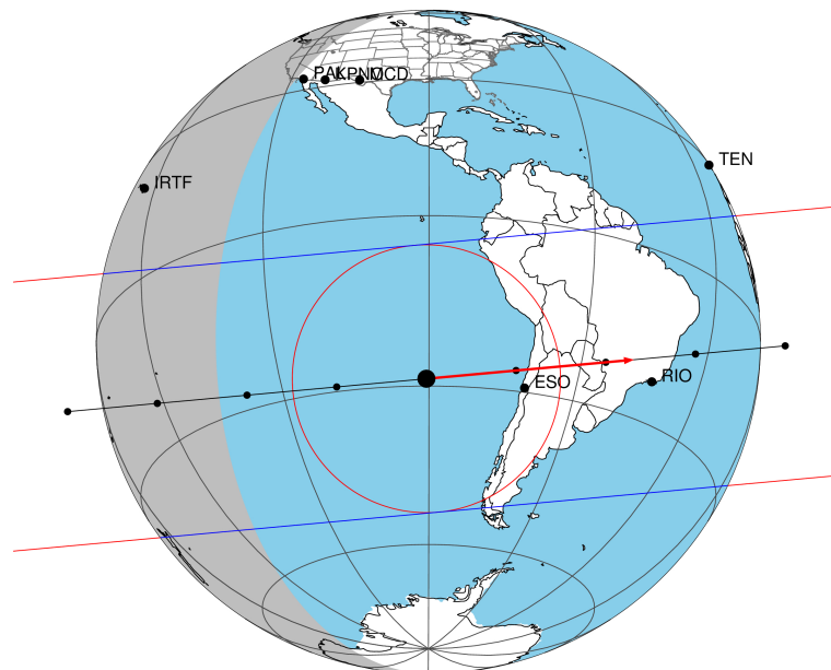
2047-02-10T14:44:49.4600 α: 18 04 05.2162 δ: -22 22 16.215 C/A 0.091" PA 174.70 deg v_sky +28.83 km/s D 10.65 AU Credit: Styled after SORA/Lucky Star
