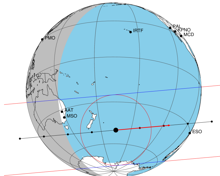
2047-02-10T19:52:40.1000 α: 18 04 10.1957 δ: -22 22 09.674 C/A 0.376" PA 174.90 deg v_sky +29.18 km/s D 10.65 AU Credit: Styled after SORA/Lucky Star
