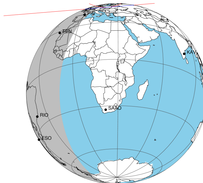
2047-02-11T06:45:21.3000 α: 18 04 20.9738 δ: -22 21 58.322 C/A 1.129" PA 355.28 deg v_sky +29.92 km/s D 10.64 AU Credit: Styled after SORA/Lucky Star
