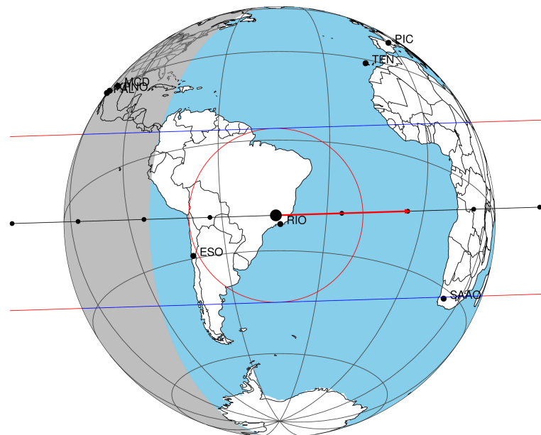
2047-02-13T11:28:01.5400 α: 18 05 16.5894 δ: -22 21 12.124 C/A 0.026" PA 358.13 deg v_sky +32.52 km/s D 10.62 AU Credit: Styled after SORA/Lucky Star
