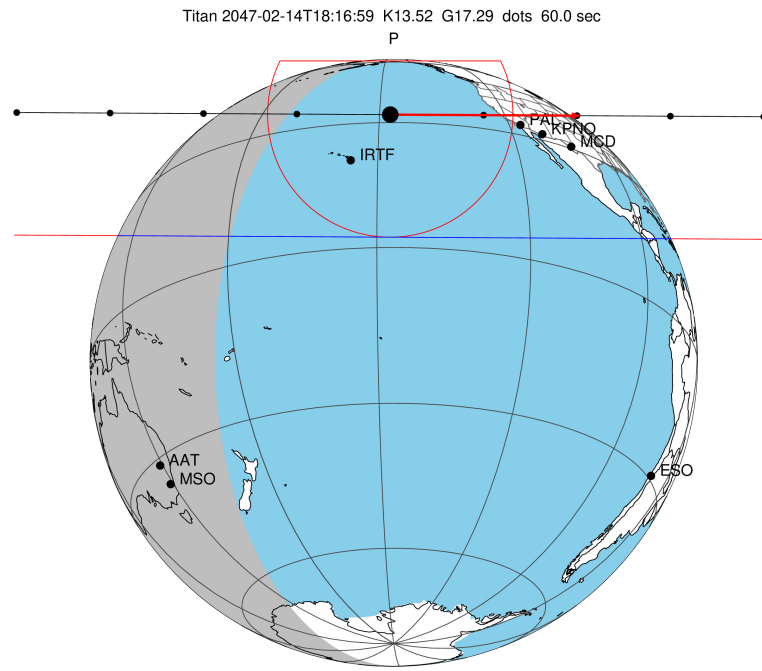
2047-02-14T18:16:59.4200 α: 18 05 50.5747 δ: -22 21 06.715 C/A 0.678" PA 0.32 deg v_sky +32.68 km/s D 10.60 AU Credit: Styled after SORA/Lucky Star
