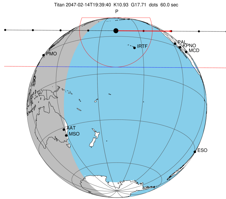
2047-02-14T19:39:40.0100 α: 18 05 52.0938 δ: -22 21 06.880 C/A 0.708" PA 0.42 deg v_sky +32.65 km/s D 10.60 AU Credit: Styled after SORA/Lucky Star
