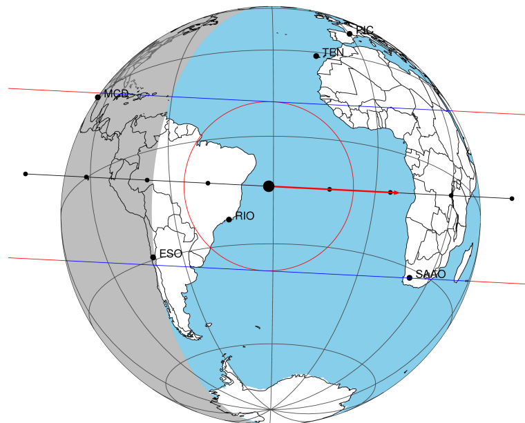
2047-02-16T10:27:00.7300 α: 18 06 33.9224 δ: -22 21 23.406 C/A 0.117" PA 2.90 deg v_sky +30.84 km/s D 10.58 AU
