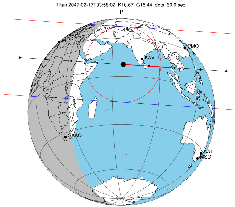
2047-02-17T03:58:02.2200 α: 18 06 51.7556 δ: -22 21 38.276 C/A 0.422" PA 3.80 deg v_sky +29.36 km/s D 10.56 AU Credit: Styled after SORA/Lucky Star
