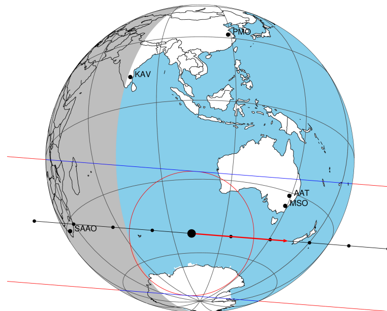
2047-02-18T01:12:31.7200 α: 18 07 12.0746 δ: -22 21 58.094 C/A 0.407" PA 184.50 deg v_sky +27.17 km/s D 10.55 AU
