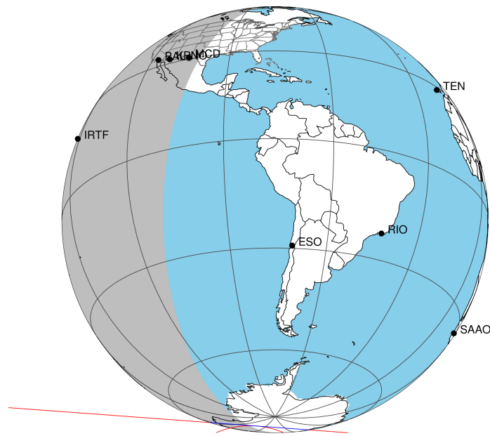
2047-02-19T13:16:47.6000 α: 18 07 42.7826 δ: -22 22 31.313 C/A 1.150" PA 184.24 deg v_sky +23.14 km/s D 10.52 AU Credit: Styled after SORA/Lucky Star
