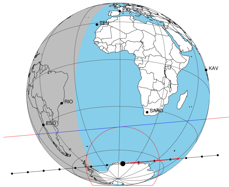
2047-02-23T08:03:57.6600 α: 18 08 44.0684 δ: -22 22 36.461 C/A 0.640" PA 174.87 deg v_sky +18.46 km/s D 10.46 AU Credit: Styled after SORA/Lucky Star
