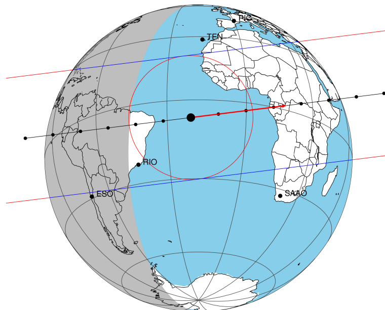
2047-02-24T09:07:41.3600 α: 18 09 00.0764 δ: -22 22 13.012 C/A 0.226" PA 352.84 deg v_sky +19.21 km/s D 10.45 AU Credit: Styled after SORA/Lucky Star
