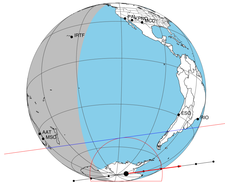
2047-02-25T16:04:30.55000 α: 18 09 21.0821 δ: -22 21 32.664 C/A 0.773" PA 172.10 deg v_sky +20.89 km/s D 10.43 AU Credit: Styled after SORA/Lucky Star
