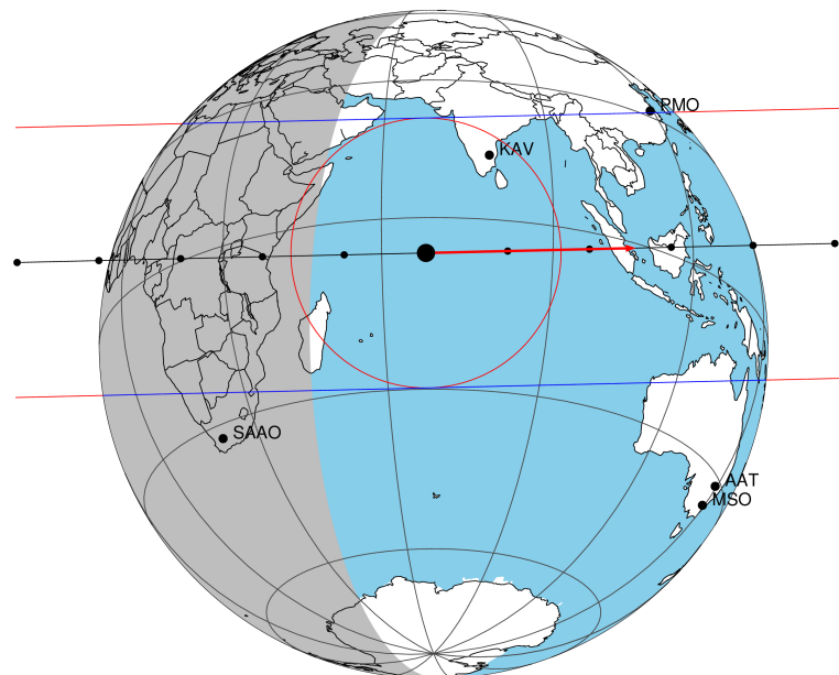
2047-03-02T02:58:13.4600 α: 18 10 48.8714 δ: -22 19 43.109 C/A 0.232" PA 358.65 deg v_sky +26.00 km/s D 10.38 AU Credit: Styled after SORA/Lucky Star
