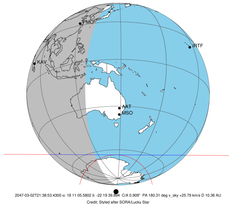
Titan 2047-03-02T21:38:53 K13.19 G17.50 dots 60.0 sec P
