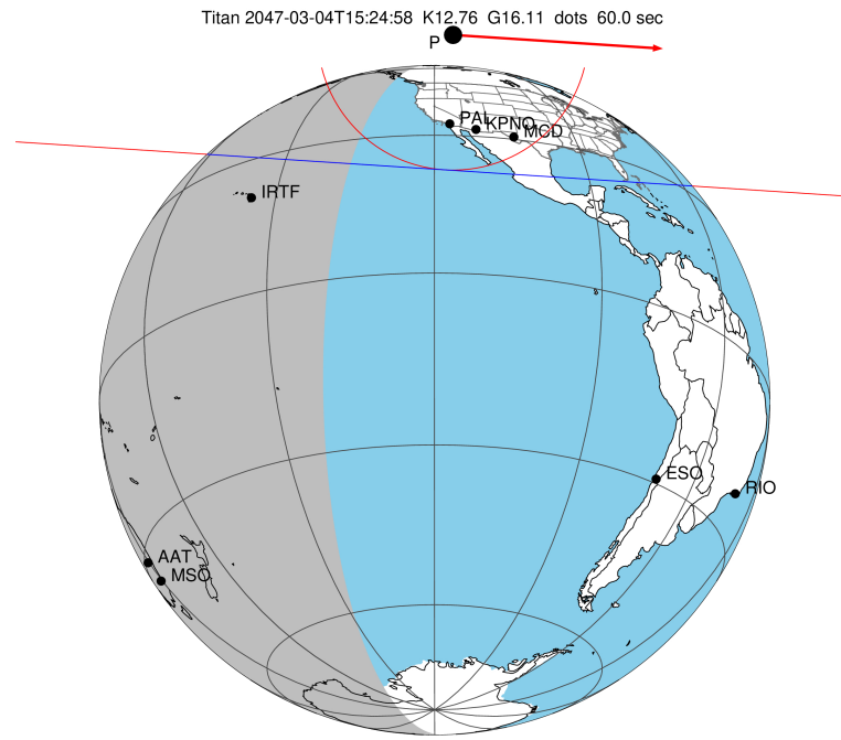
2047-03-04T15:24:58.5900 α: 18 11 41.4398 δ: -22 19 59.563 C/A 0.929" PA 3.74 deg v_sky +23.52 km/s D 10.34 AU Credit: Styled after SORA/Lucky Star
