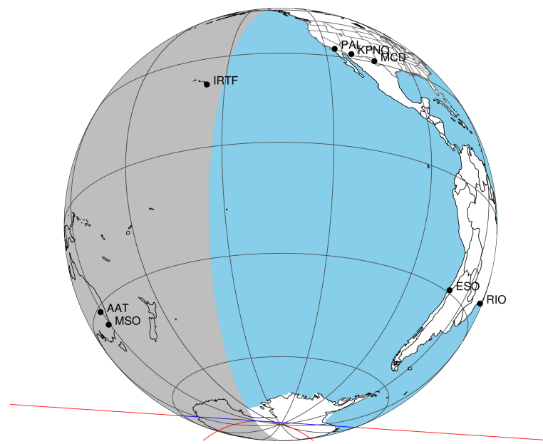
2047-03-04T16:21:58.5300 α: 18 11 42.2201 δ: -22 19 58.223 C/A 1.121" PA 183.82 deg v_sky +23.44 km/s D 10.33 AU Credit: Styled after SORA/Lucky Star
