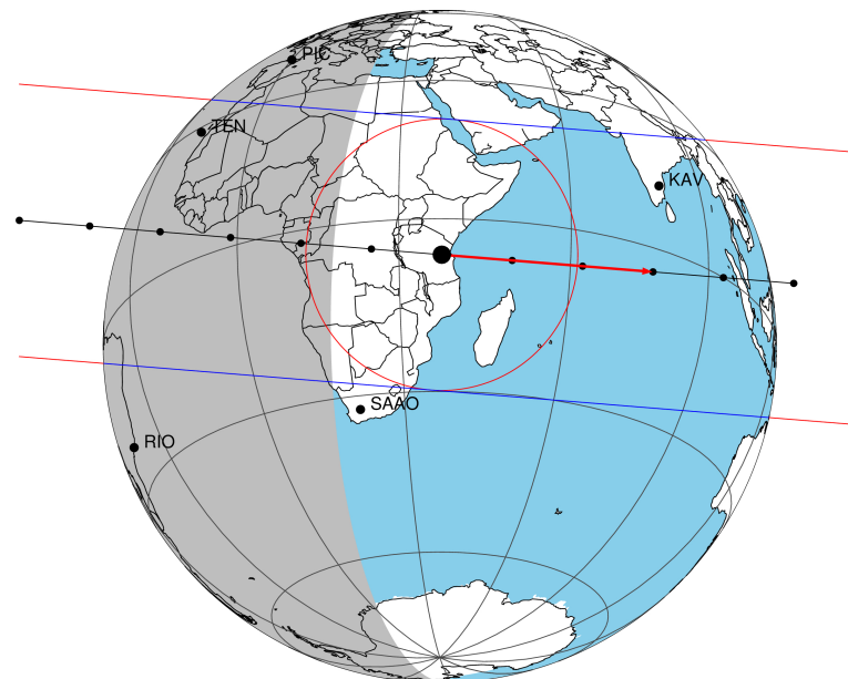
2047-03-05T04:55:01.2300 α: 18 11 52.1333 δ: -22 20 09.785 C/A 0.232" PA 4.65 deg v_sky +22.30 km/s D 10.32 AU Credit: Styled after SORA/Lucky Star
