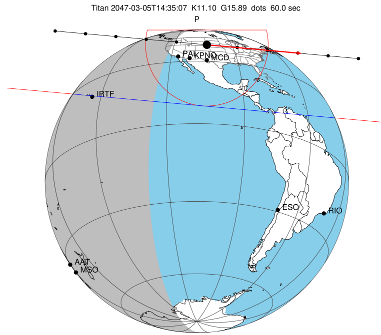
2047-03-05T14:35:07.1100 α: 18 11 59.4121 δ: -22 20 19.053 C/A 0.769" PA 5.21 deg v_sky +21.31 km/s D 10.32 AU Credit: Styled after SORA/Lucky Star
