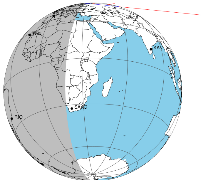
2047-03-06T04:51:31.3900 α: 18 12 09.5295 δ: -22 20 33.043 C/A 1.181" PA 5.80 deg v_sky +19.74 km/s D 10.31 AU Credit: Styled after SORA/Lucky Star
