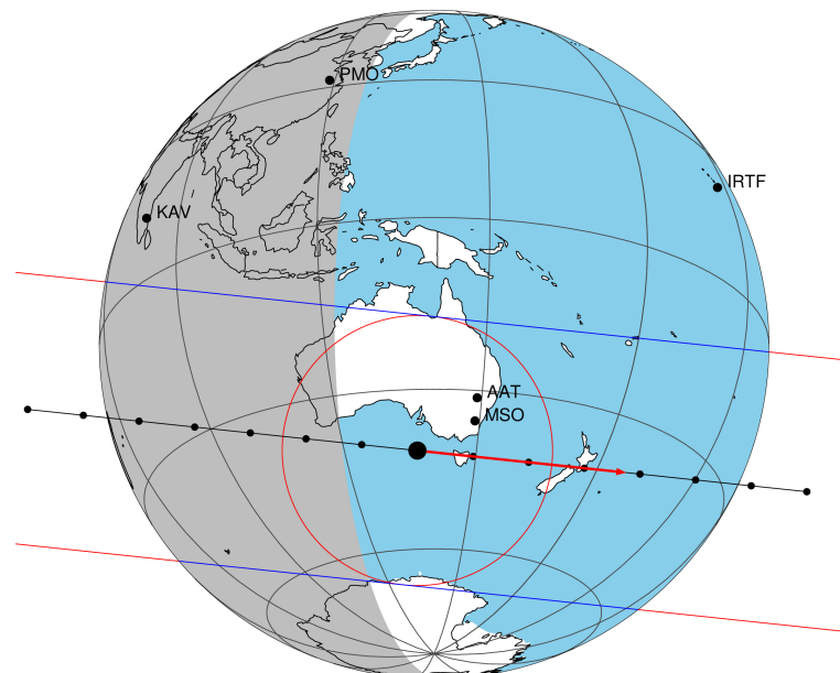
2047-03-06T21:55:10.6300 α: 18 12 20.5938 δ: -22 20 47.620 C/A 0.274" PA 186.04 deg v_sky +17.77 km/s D 10.29 AU Credit: Styled after SORA/Lucky Star
