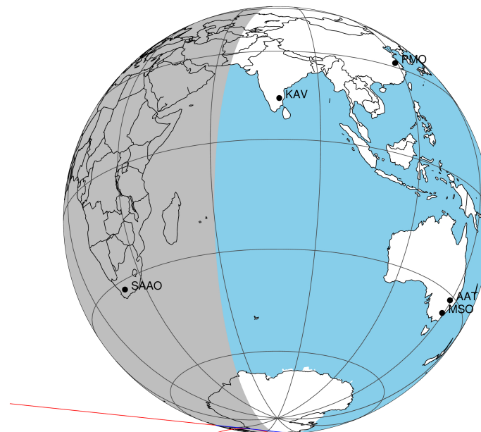
2047-03-07T02:02:59.5400 α: 18 12 23.1036 δ: -22 20 50.377 C/A 1.185" PA 186.00 deg v_sky +17.29 km/s D 10.29 AU Credit: Styled after SORA/Lucky Star
