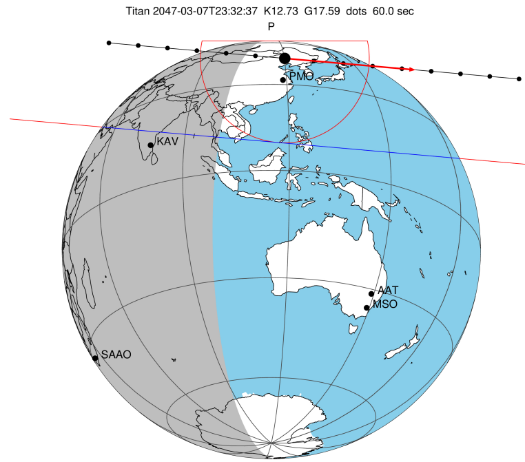
2047-03-07T23:32:37.5700 α: 18 12 35.0670 δ: -22 21 08.752 C/A 0.786" PA 5.03 deg v_sky +14.94 km/s D 10.27 AU Credit: Styled after SORA/Lucky Star
