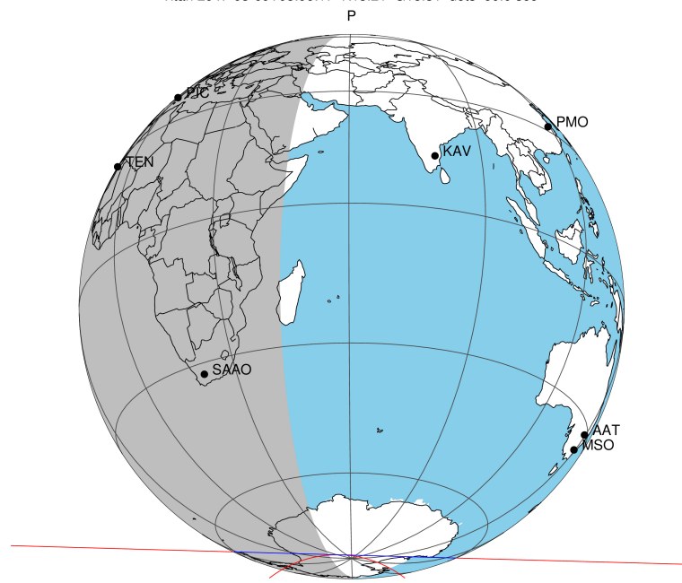
2047-03-09T03:06:17.7900 α: 18 12 48.1852 δ: -22 21 18.196 C/A 1.129" PA 181.59 deg v_sky +12.56 km/s D 10.25 AU Credit: Styled after SORA/Lucky Star
