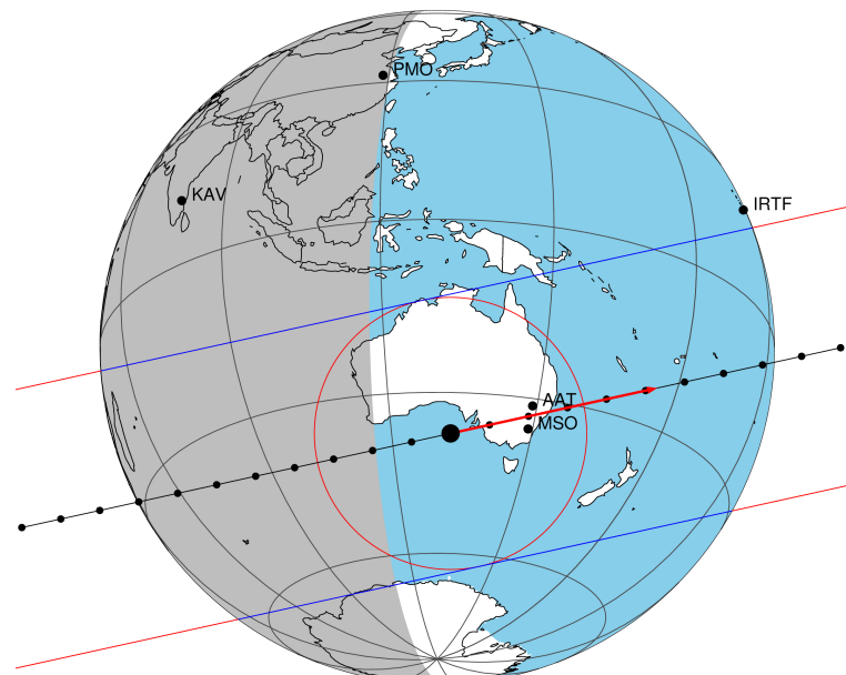
2047-03-12T22:15:14.8500 α: 18 13 24.8937 δ: -22 20 18.763 C/A 0.223" PA 167.60 deg v_sky +12.58 km/s D 10.19 AU Credit: Styled after SORA/Lucky Star
