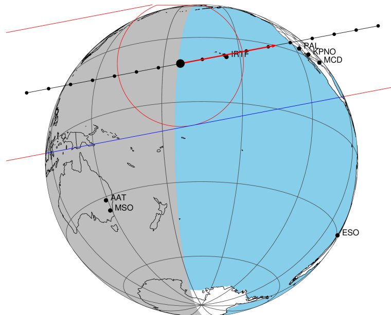
2047-03-14T17:48:19.9100 α: 18 13 45.6590 δ: -22 19 18.581 C/A 0.552" PA 349.19 deg v_sky +15.21 km/s D 10.17 AU Credit: Styled after SORA/Lucky Star
