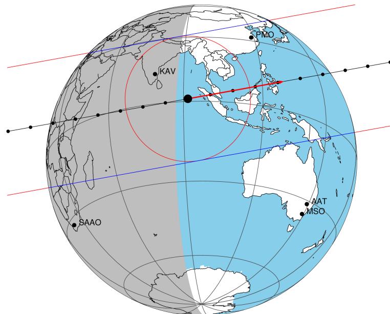
2047-03-15T00:19:39.0800 α: 18 13 49.1345 δ: -22 19 09.407 C/A 0.350" PA 349.74 deg v_sky +15.62 km/s D 10.16 AU Credit: Styled after SORA/Lucky Star
