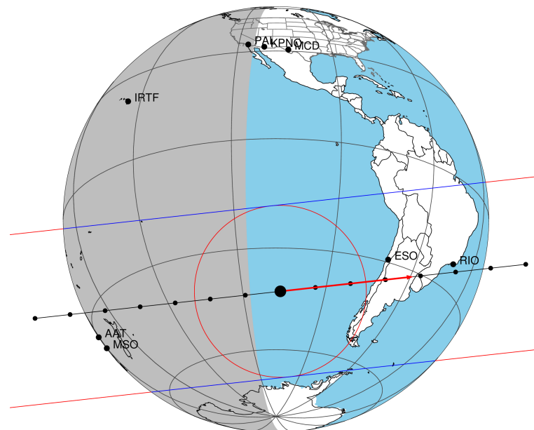
2047-03-16T13:52:09.3800 α: 18 14 10.9519 δ: -22 18 24.498 C/A 0.293" PA 173.70 deg v_sky +17.61 km/s D 10.14 AU Credit: Styled after SORA/Lucky Star
