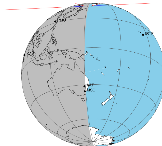
2047-03-17T20:06:10.3400 α: 18 14 30.1922 δ: -22 18 05.167 C/A 1.184" PA 357.39 deg v_sky +18.39 km/s D 10.12 AU
