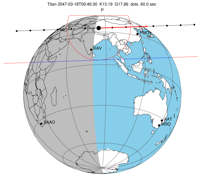
2047-03-18T00:46:30.1700 α: 18 14 33.2263 δ: -22 18 03.005 C/A 0.732" PA 357.97 deg v_sky +18.41 km/s D 10.12 AU Credit: Styled after SORA/Lucky Star
