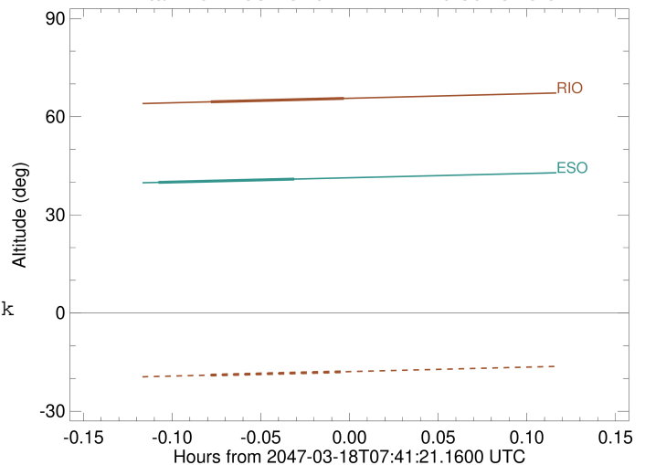
Titan 2047-03-18T07:41:21 K10.39 G16.07
