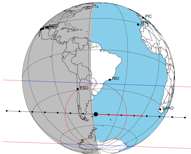
2047-03-19T10:00:18.6600 α: 18 14 54.6307 δ: -22 18 02.086 C/A 0.408" PA 182.15 deg v_sky +17.74 km/s D 10.10 AU
