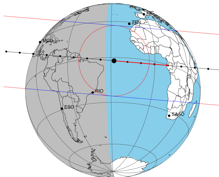
2047-03-20T08:21:32.9300 α: 18 15 08.1804 δ: -22 18 14.361 C/A 0.298" PA 4.92 deg v_sky +16.41 km/s D 10.08 AU Credit: Styled after SORA/Lucky Star
