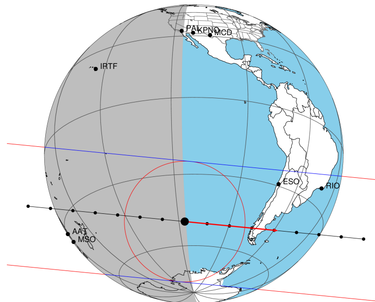
2047-03-20T13:50:55.4800 α: 18 15 11.3275 δ: -22 18 17.677 C/A 0.397" PA 185.58 deg v_sky +15.98 km/s D 10.08 AU Credit: Styled after SORA/Lucky Star
