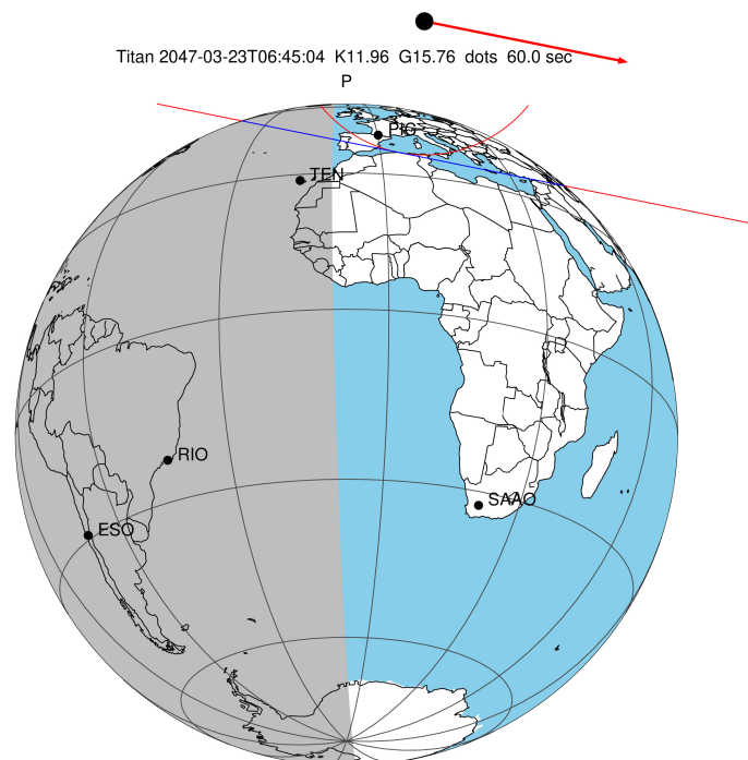
2047-03-23T06:45:04.0000 α: 18 15 40.2630 δ: -22 19 20.650 C/A 1.115" PA 11.38 deg v_sky + 9.04 km/s D 10.02 AU Credit: Styled after SORA/Lucky Star
