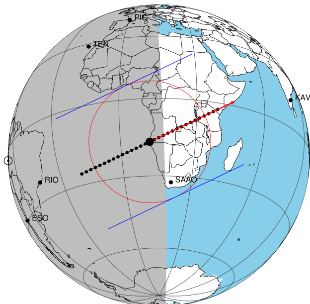
2047-03-27T04:58:49.3200 cc: 18 15 57.3065 d: -22 19 31.348 C/A 0.096" PA 334.62 deg v_sky + 3.53 km/s D 09.95 AU Credit: Styled after SORA/Lucky Star
