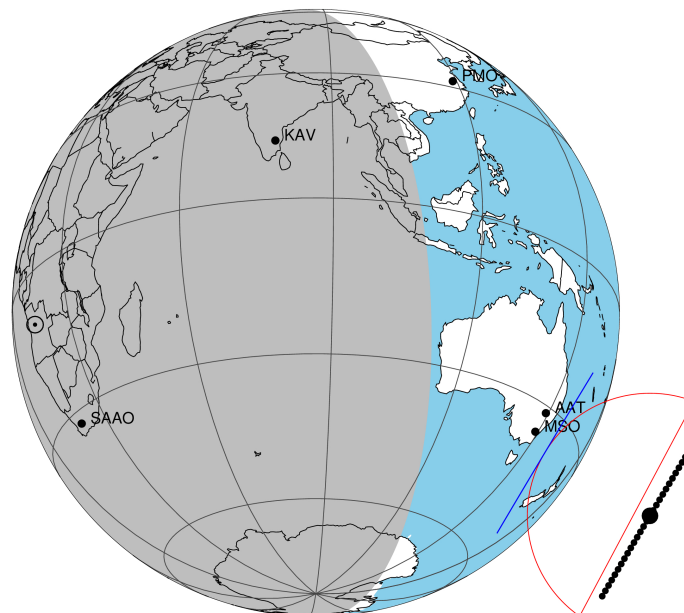
2047-04-16T22:52:50.6800 ra: 18 16 50.0103 d: -22 16 24.337 C/A 1.176" PA 120.91 deg v_sky + 2.18 km/s D 09.63 AU Credit: Styled after SORA/Lucky Star
