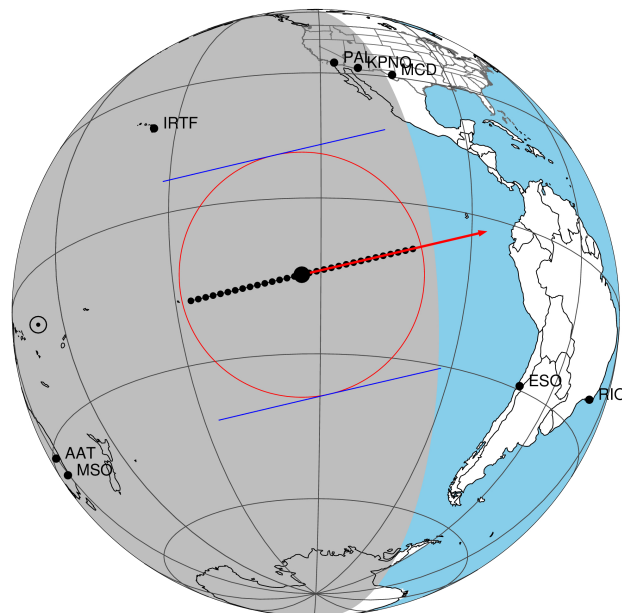
2047-04-18T12:37:22.2900 α: 18 16 52.8525 δ: -22 16 00.121 C/A 0.122" PA 346.84 deg v_sky + 2.66 km/s D 09.60 AU Credit: Styled after SORA/Lucky Star
