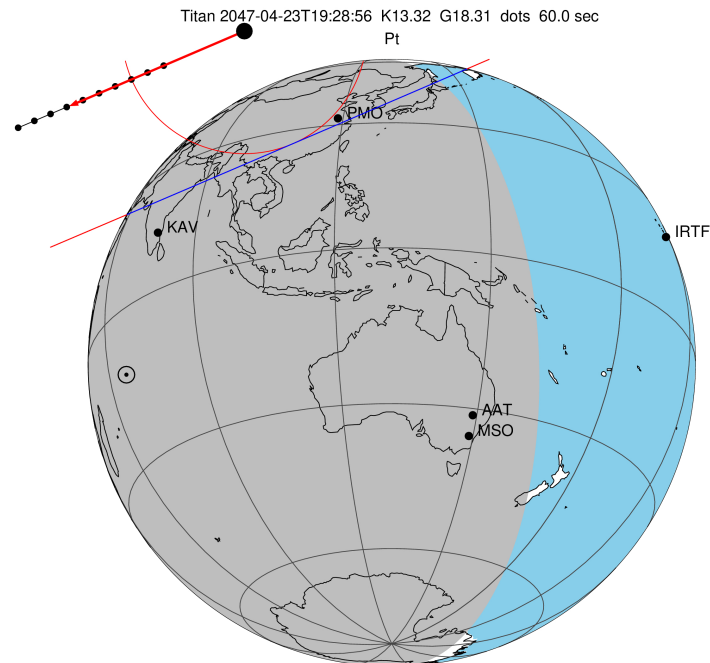
2047-04-23T19:28:56.5000 α: 18 16 53.0214 δ: -22 17 40.087 C/A 1.105" PA 336.79 deg v_sky - 6.14 km/s D 09.52 AU Credit: Styled after SORA/Lucky Star
