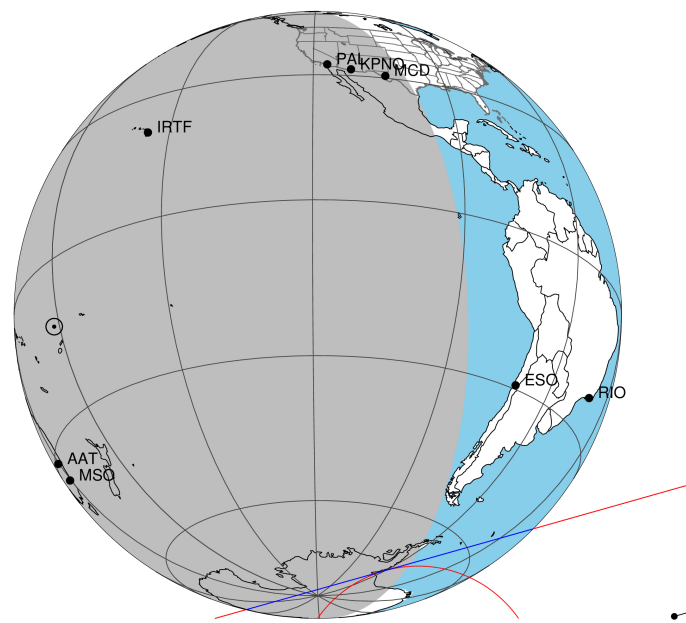
2047-04-24T12:05:44.4600 α: 18 16 48.8610 δ: -22 17 57.687 C/A 1.179" PA 164.27 deg v_sky - 7.77 km/s D 09.51 AU
