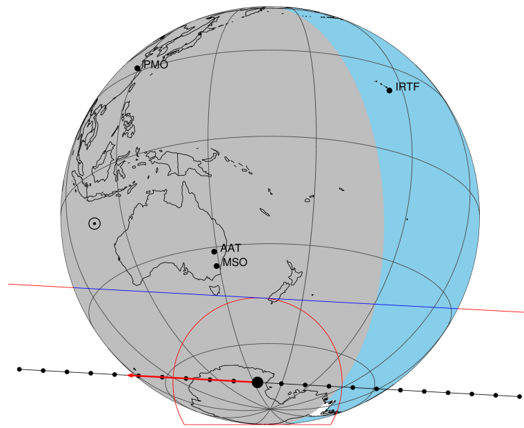
2047-04-27T16:47:32.4500 α: 18 16 18.6293 δ: -22 18 30.458 C/A 0.743" PA 183.13 deg v_sky -12.11 km/s D 09.46 AU Credit: Styled after SORA/Lucky Star
