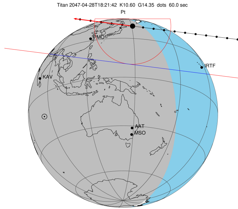
2047-04-28T18:21:42.3900 α: 18 16 07.0026 δ: -22 18 17.247 C/A 0.861" PA 7.28 deg v_sky -11.86 km/s D 09.44 AU Credit: Styled after SORA/Lucky Star
