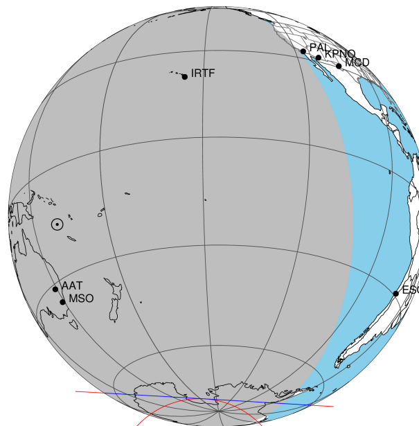
2047-05-04T13:11:07.5200 α: 18 15 25.1560 δ: -22 16 09.307 C/A 1.193" PA 183.37 deg v_sky - 4.35 km/s D 09.38 AU
