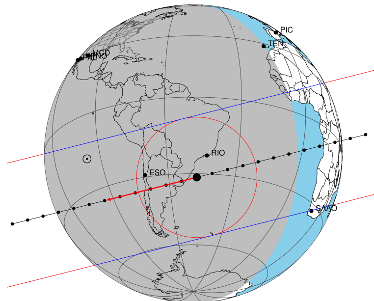
2047-05-09T06:25:19.1000 cc: 18 14 57.7799 s: -22 17 52.865 C/A 0.151" PA 165.79 deg v_sky -11.30 km/s D 09.31 AU Credit: Styled after SORA/Lucky Star
