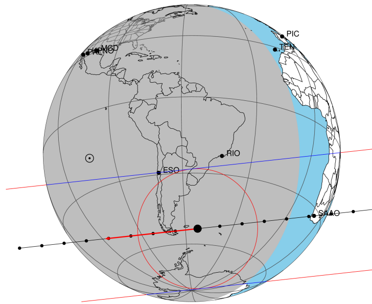
2047-05-11T06:45:07.6000 cc: 18 14 32.5866 d: -22 18 53.843 C/A 0.483" PA 173.74 deg v_sky -16.00 km/s D 09.28 AU Credit: Styled after SORA/Lucky Star
